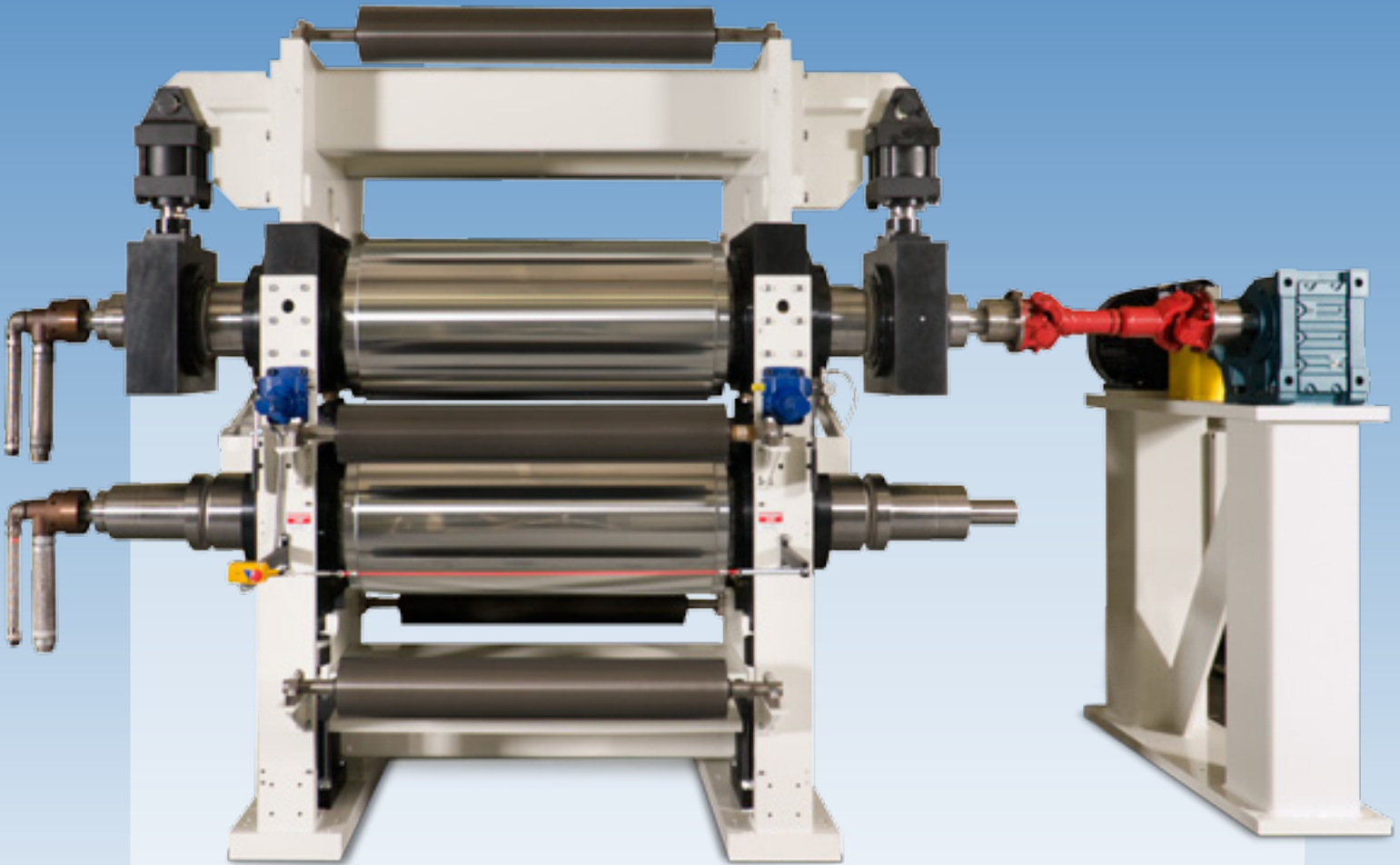
Heated Calender with Roll Bending
