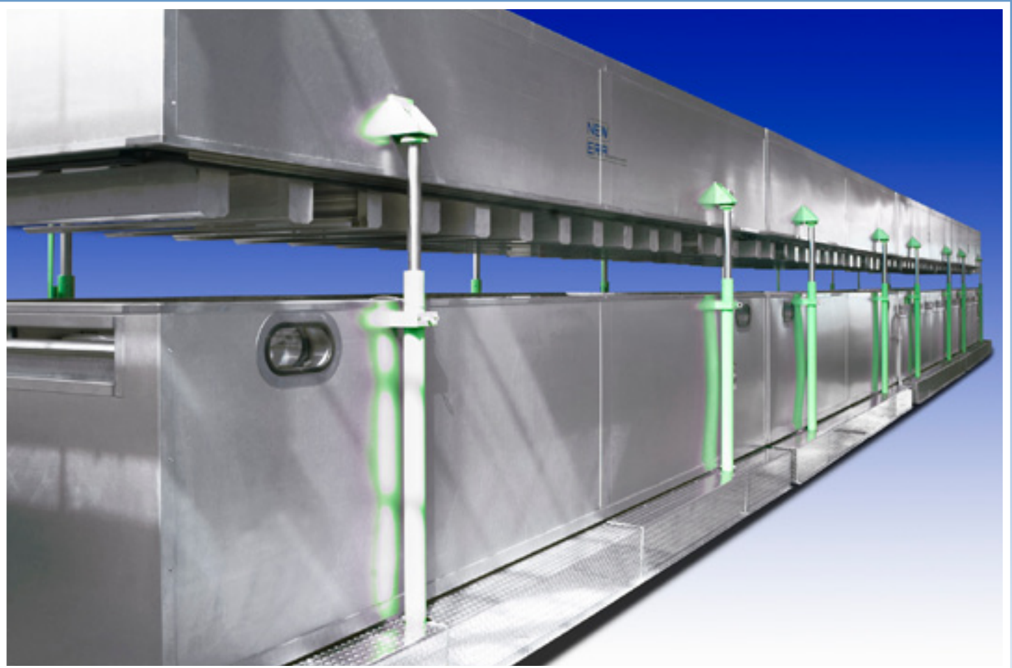
Four Zone Electrically Heated Air Floatation Dryer
